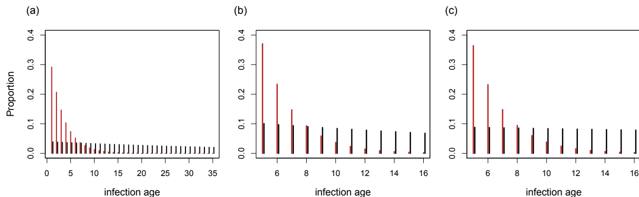
Figure B-1: Average stable age distributions, q(s) , in epidemic (red) and endemic (black scenarios). Shown are the average distributions across 10000 bootstrap replicates for infections in (a) C57 mice, (b) C57 mice, truncated data set, (c) MF1 mice.
